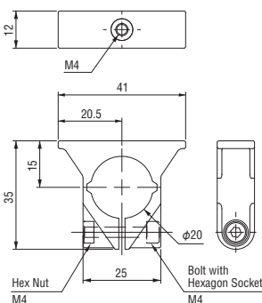
Resin Fixture φ 20 (M4)
