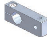
Suction bracket • φ 12 • M5
