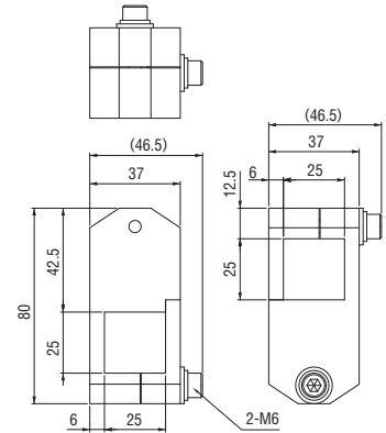
Slide bracket • 10-20
