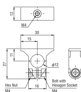
Resin Fixture φ 12 (M4)
