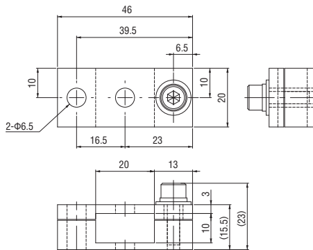
Slide bracket • 20-10
