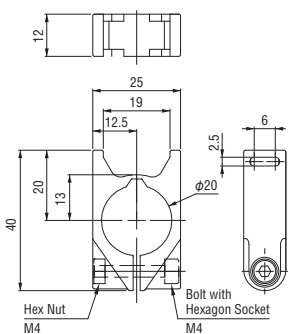
Resin Fixture φ 20 (Cable ties)
