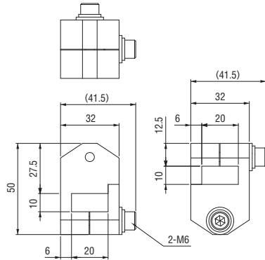
Attachment bracket • 10-20 • M6
